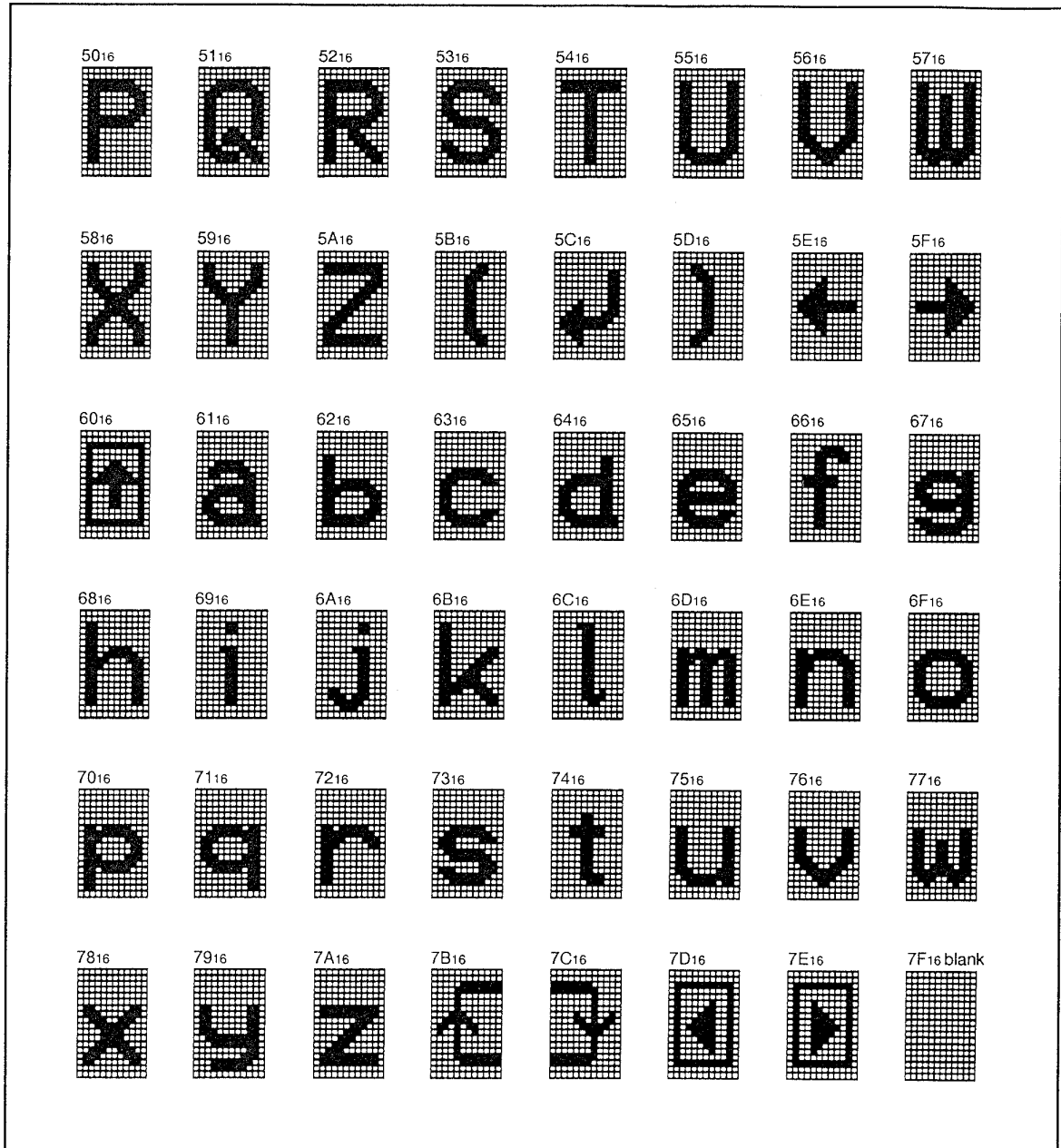
Fig. 13 M35043-001SP/FP character patterns (3)
